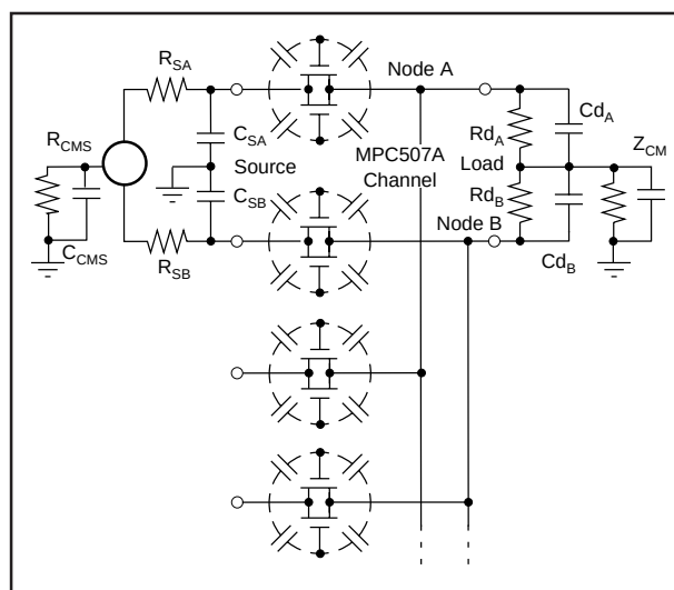
FIGURE 4. Settling and Common-Mode Effects—MPC507A
